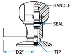
INLET - CONC. TC; OUTLET - TUBE;
