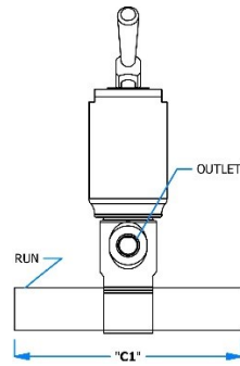
INLET - AUTOWELDED RUN; OUTLET - HOSE BARB;
