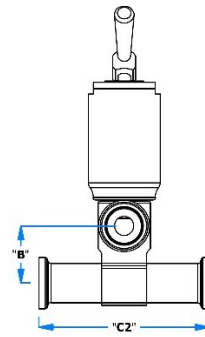
INLET - TC RUN; OUTLET - TC;
