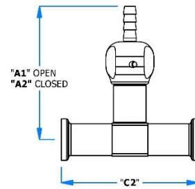
INLET – TC RUN; OUTLET – HOSE BARB;
