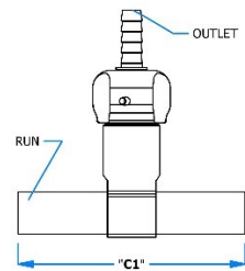
INLET – AUTOWELDED RUN; OUTLET – HOSE BARB;
